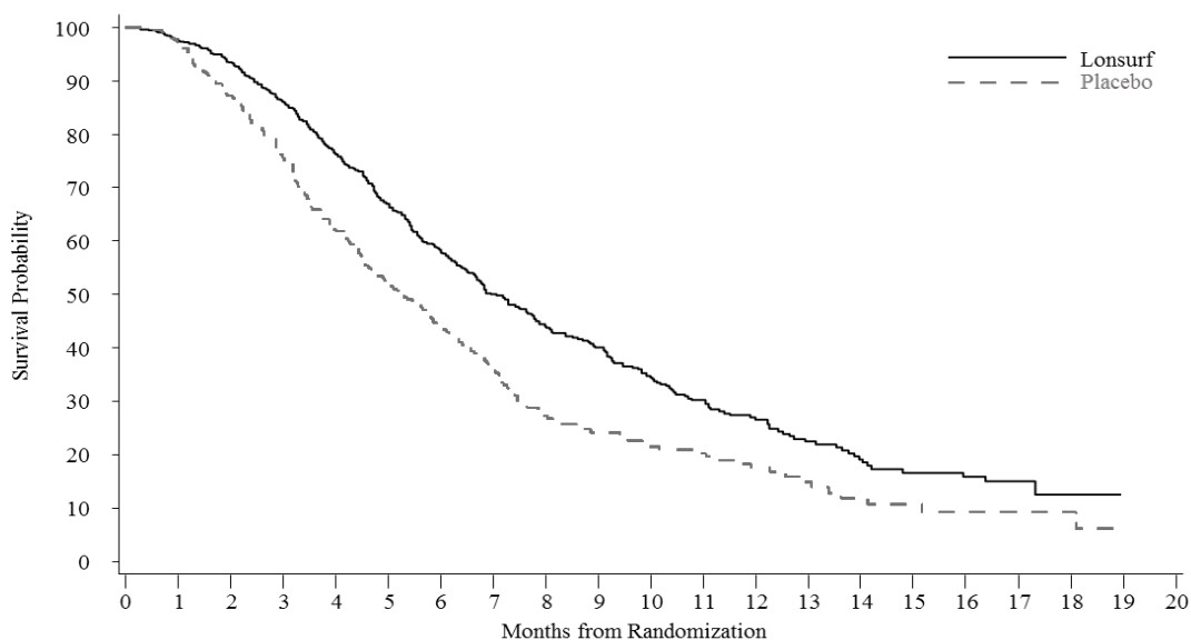
Figure 1 Kaplan-Meier Curves of Overall Survival in RECOURSE
